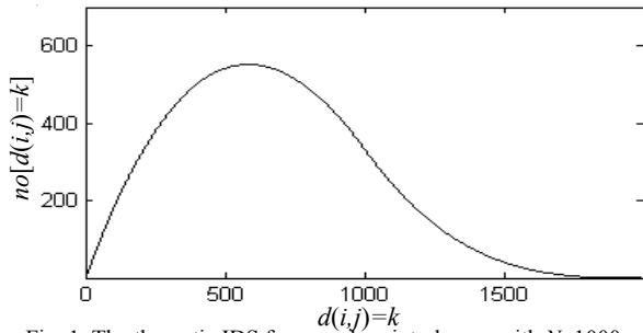
Fig. 1. The theoretic IDS for a random interleaver with N=1000 .
