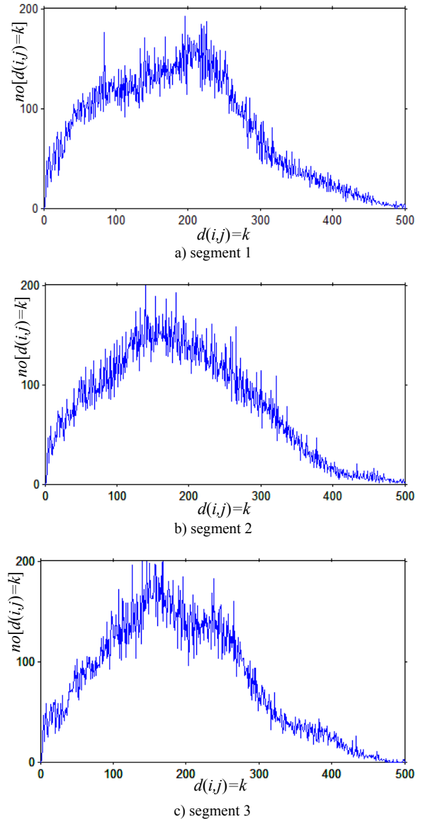
Fig. 3. The IDS for the sets of 280 frequencies which constitute the resource allocated to the 3 segments in the DLPUSC 1024 case.
