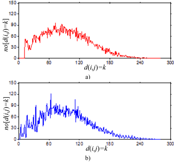
Fig. 2. The DS for: a) the S -interleaver with S=13 and N=140 ; b) the permutation system defined by the positions sequence of the 140 sub-carrier frequencies of BS segment 0.
